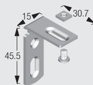
Bracket for mounting profile 305001052 white 305000752 galvanised
